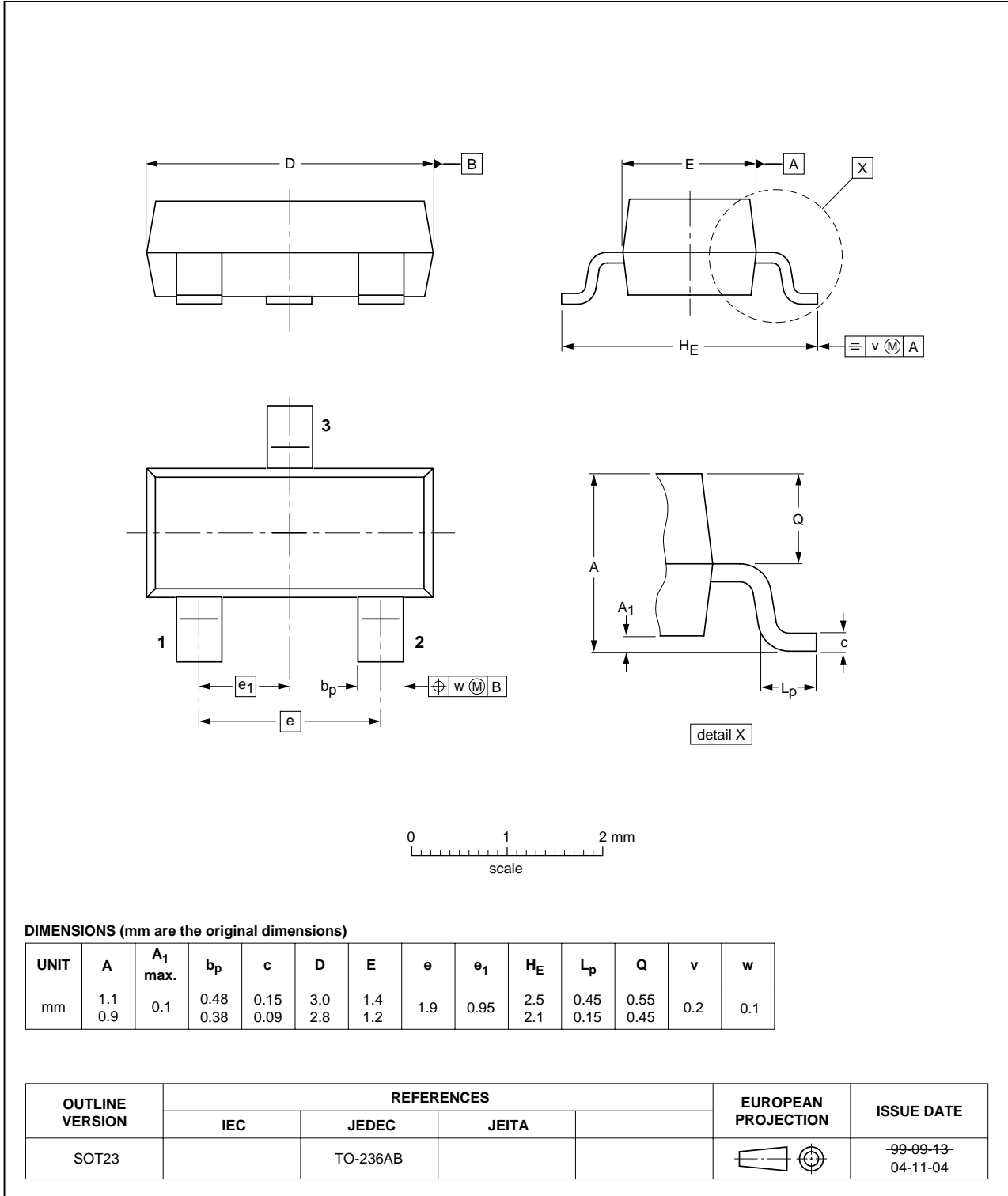
www.DataSheet4U.com Fig 14. Package outline SOT23
