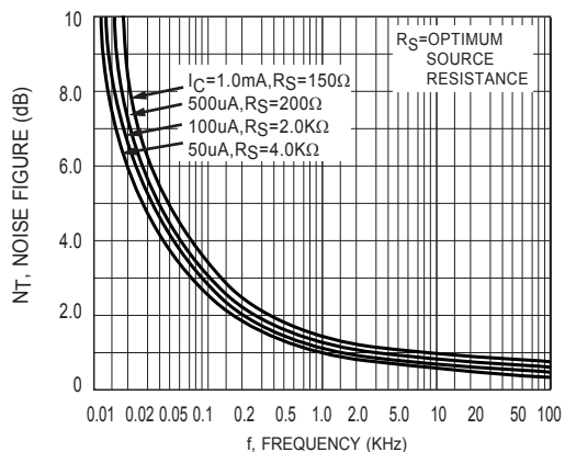
Figure 5. Frequency Effects
