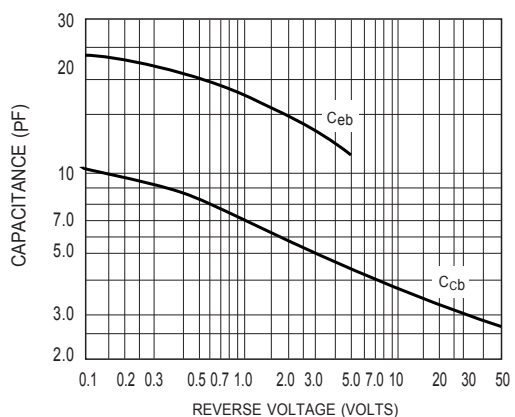
Figure 7. Capacitances
