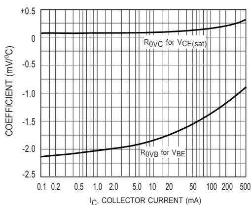
Figure 10. Temperature Coefficients
