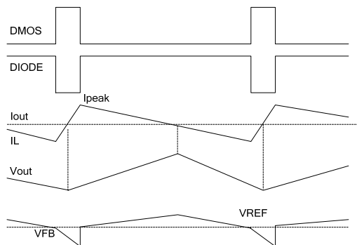
Figure 1-1 Waveform of CCM mode
