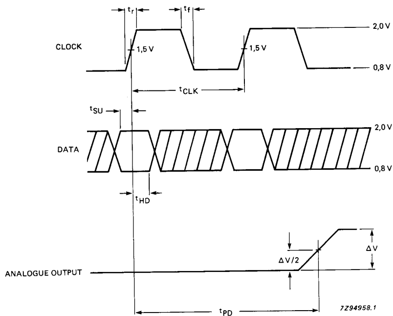
Fig. 3 Switching characteristics.
