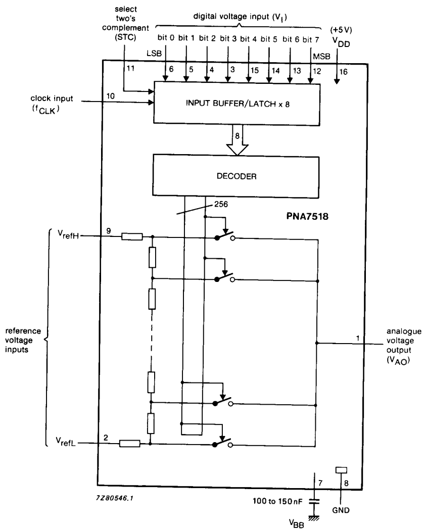
Fig. 1 Block diagram.
