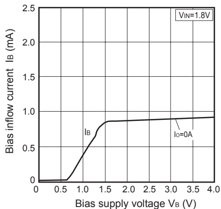
Fig.28 Bias Inflow Current vs. Bias Supply Voltage (PQ012GN1HZPH)
