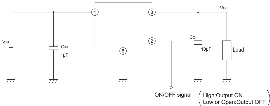
Fig.1 Typical Application
