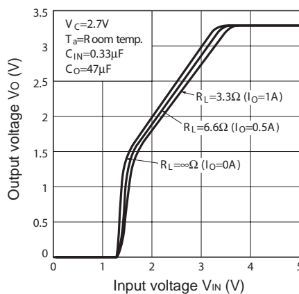
Fig.28 Output Voltage vs. Input Voltage (PQ033EZ01ZxH)
