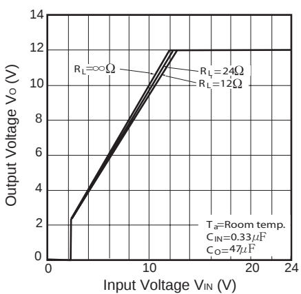
Fig.13 Output Voltage vs. Input Voltage (PQ120RDA1SZH)
