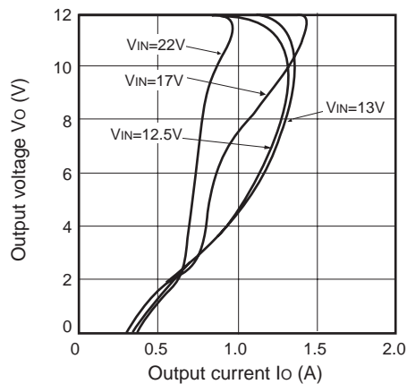
Fig.8 Overcurrent Protection Characteristics (PQ120RDA1SZH)
