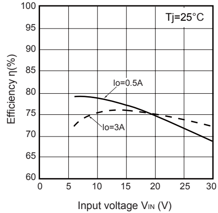
Fig.5 Efficiency vs. Input Voltage (PQ1CY333LHZPH)
