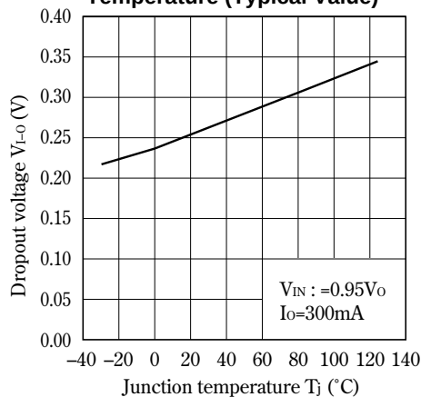
Fig.8 Dropout Voltage vs. Junction Temperature (Typical Value)
