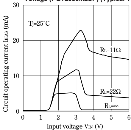
Fig.7 Circuit Operating Current vs. Input Voltage (PQ1L333M2SP) (Typical Value)
