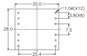
PCB PATTERN
