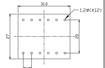
PCB PATTERN
