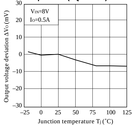
Fig.10 Output Voltage Deviation vs. Junction Temperature (PQ6RD083)
