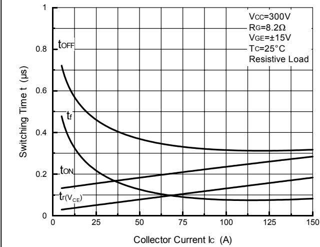
Fig.7- Collector Current vs. Switching Time (Typical)
