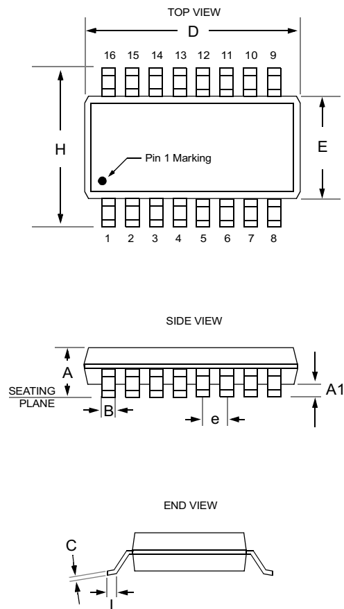
Package Dimensions for SOIC-16 (Wide)
