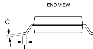
Package Dimensions for QSOP-20
