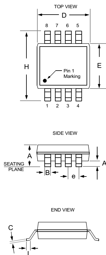
Package Dimensions for SOIC-8
