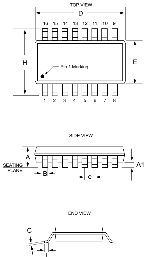
Package Dimensions for SOIC-16 (Narrow)
