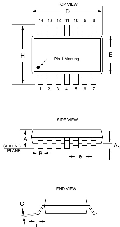
Package Dimensions for SOIC-14
