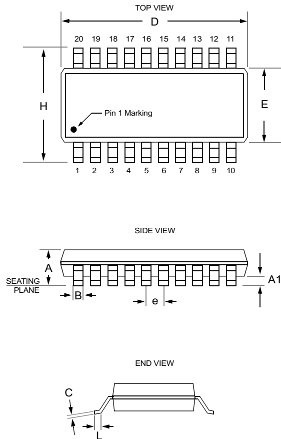
Package Dimensions for SOIC-20
