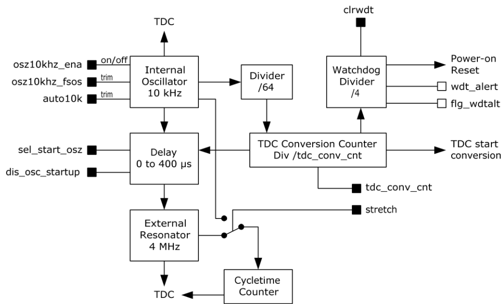
Figure 3-1: Clock Generation
