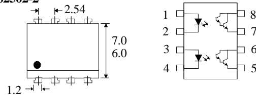
PS2502-2X PS2502-2
