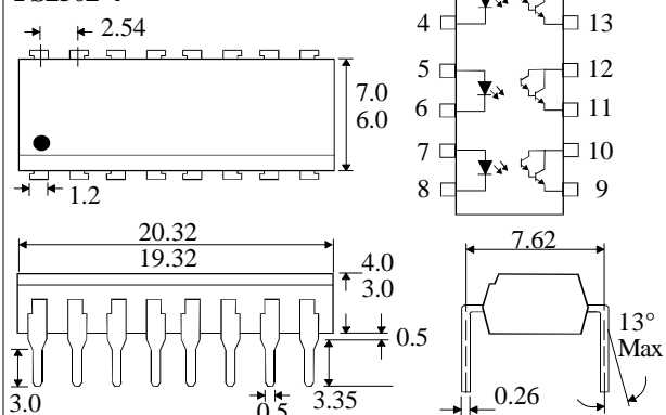
PS2502-4X PS2502-4
