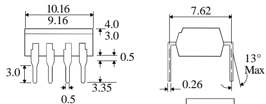
PS2502-4X PS2502-4
