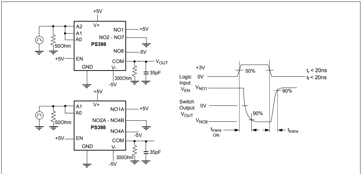
Figure 1. Transition Time
