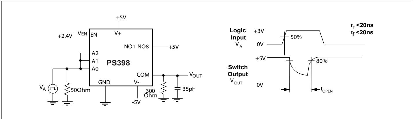
Figure 3. Break-Before-Make Interval
