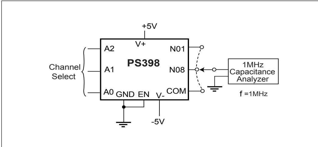
Figure 8. NO/COM Capacitance
