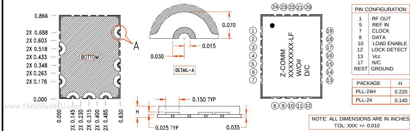
PHYSICAL DIMENSIONS
