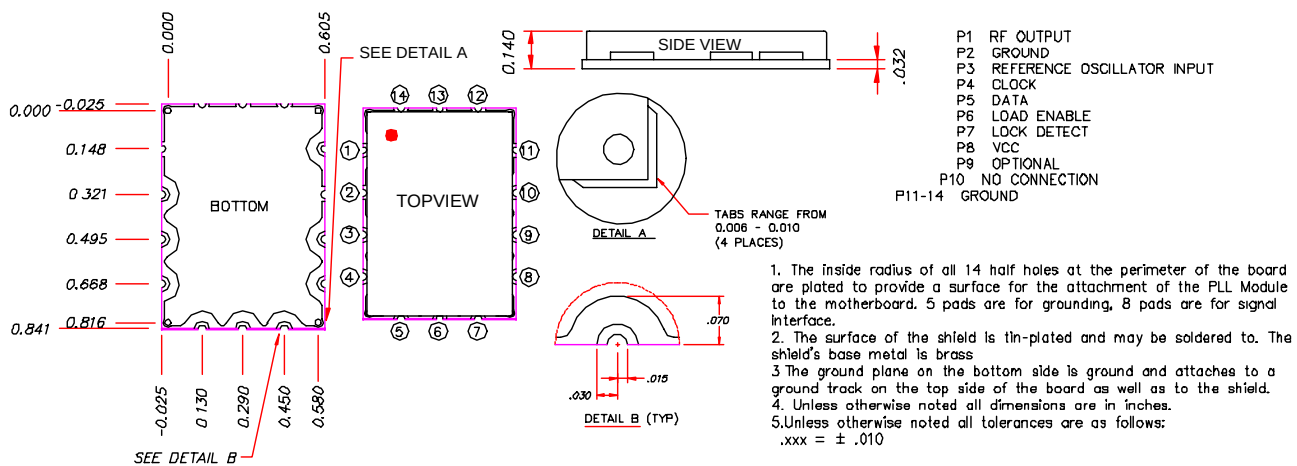
PHYSICAL DIMENSIONS
