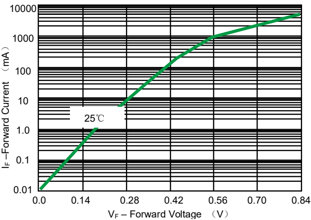
Fig 1.Forward Voltage
