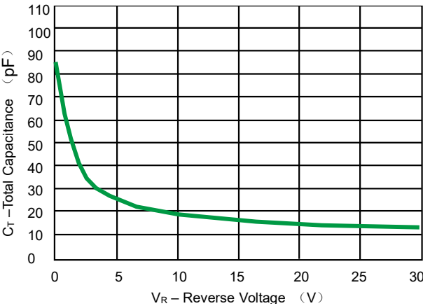
Fig 3.Total Capacitance
