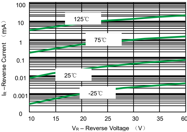
Fig 2.Leakage Current
