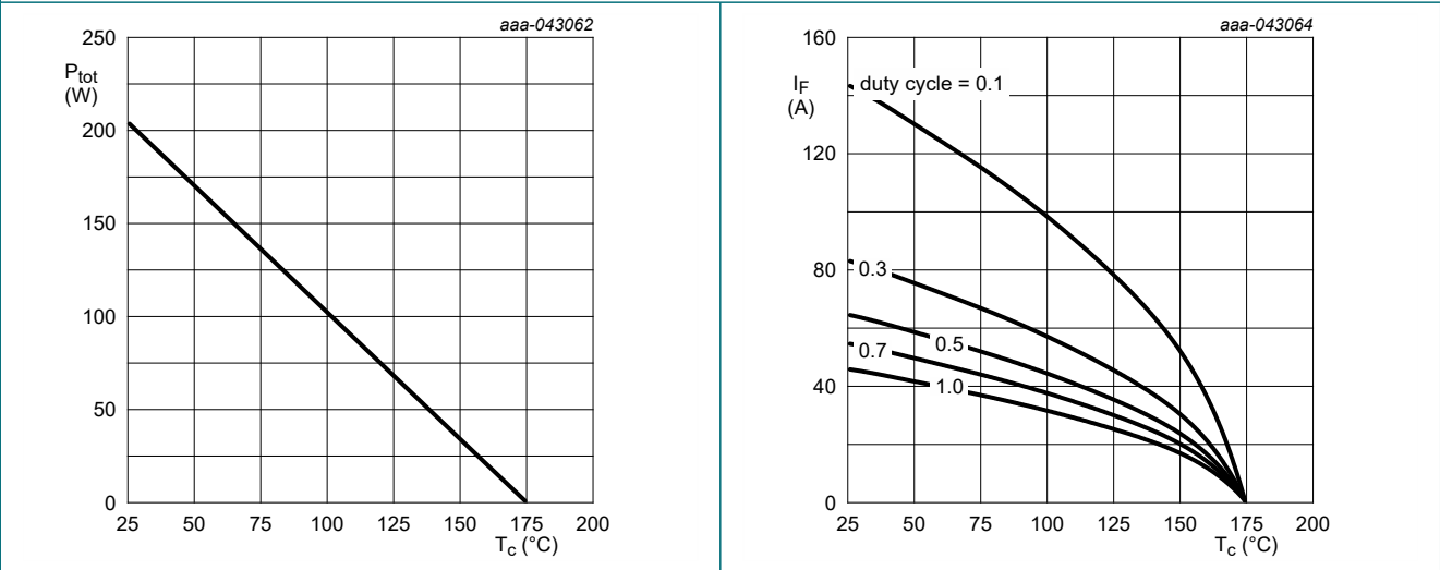
Fig. 2. Power dissipation; maximum values
