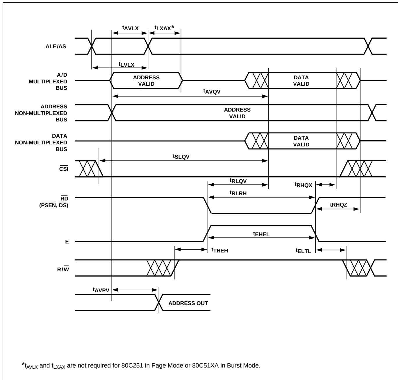
Figure 34. Read Timing
