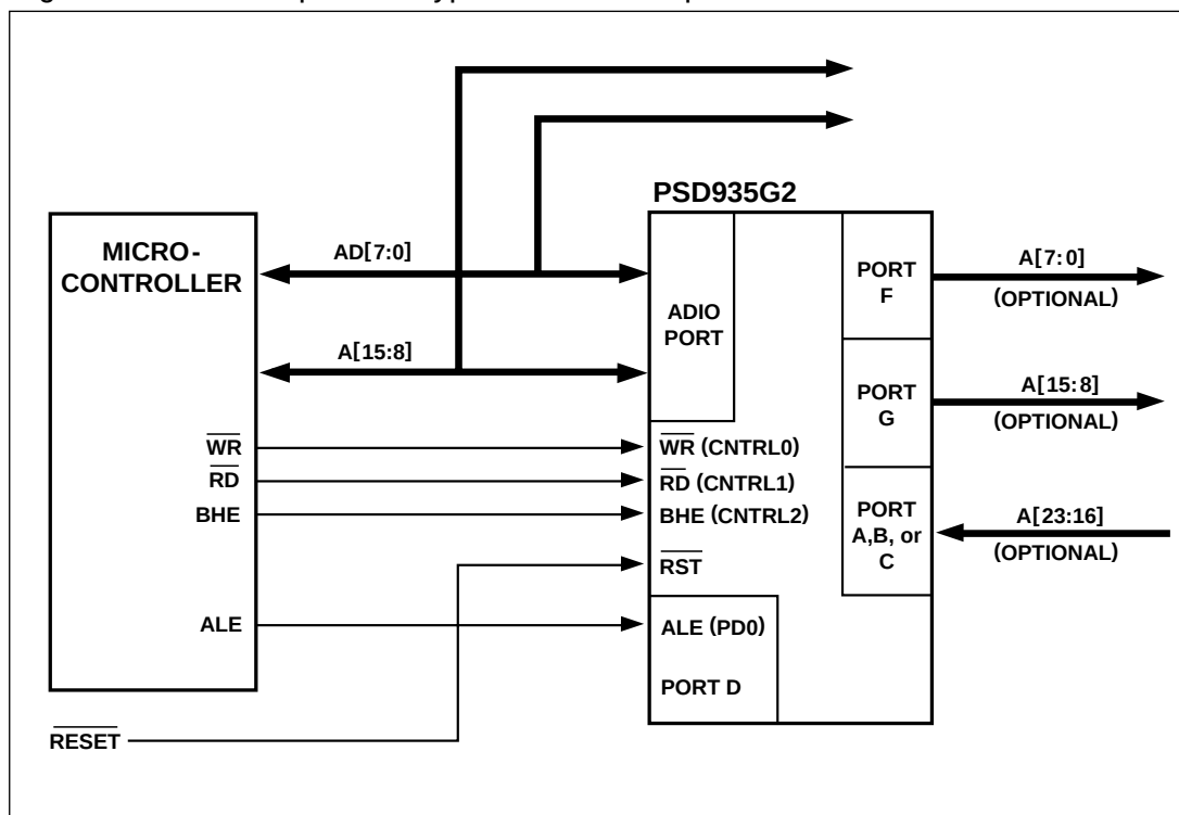
Figure 13. An Example of a Typical 8-Bit Multiplexed Bus Interface
