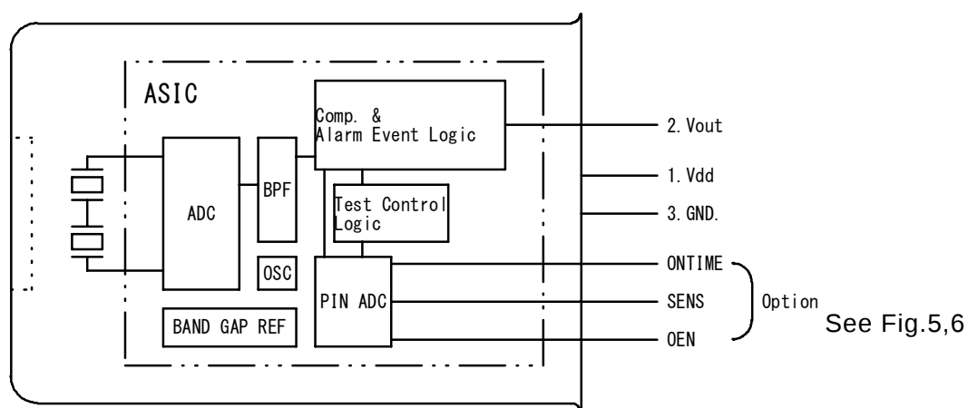
Fig.3 : Circuit Configuration
