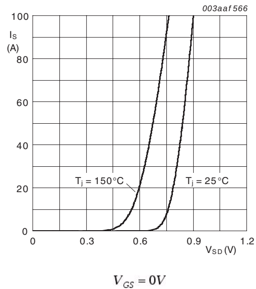
Fig 17. Source current as a function of drain-source voltage; typical values
