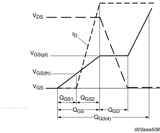
Fig 14. Gate charge waveform definitions
