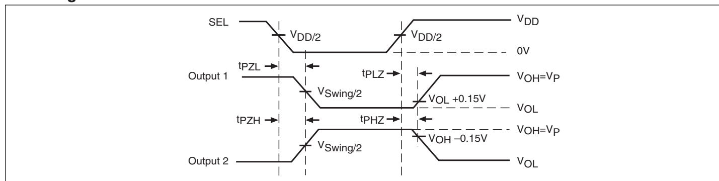
Figure 6. Voltage Waveforms Enable and Disable Times
