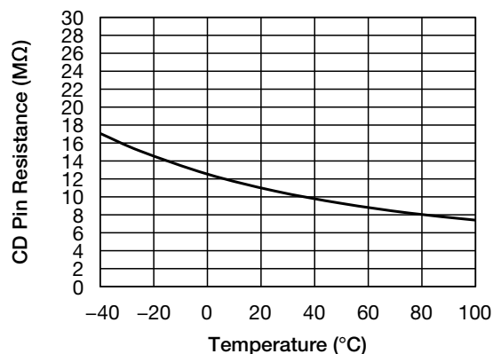
CD Pin Resistance - Temperature
