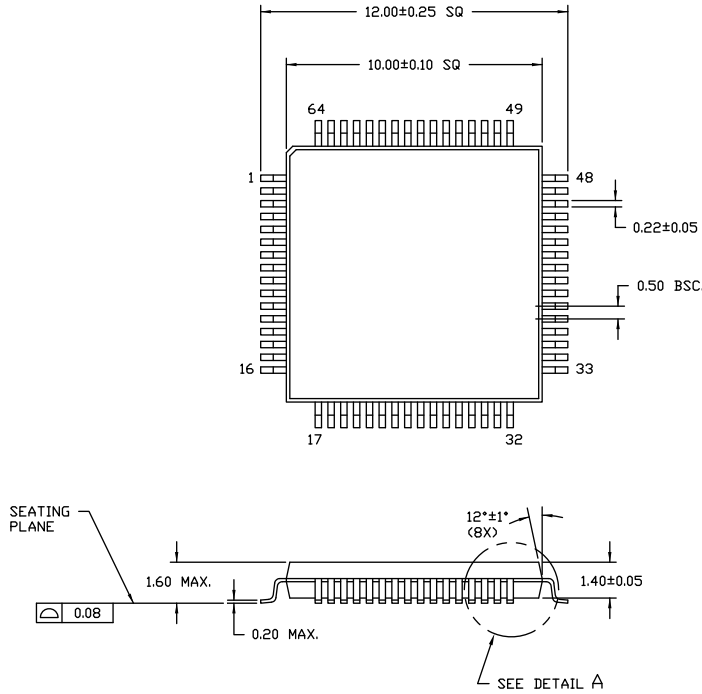
Figure 5. 64-Pin 10 × 10 × 1.4 mm TQFP Package Outline
