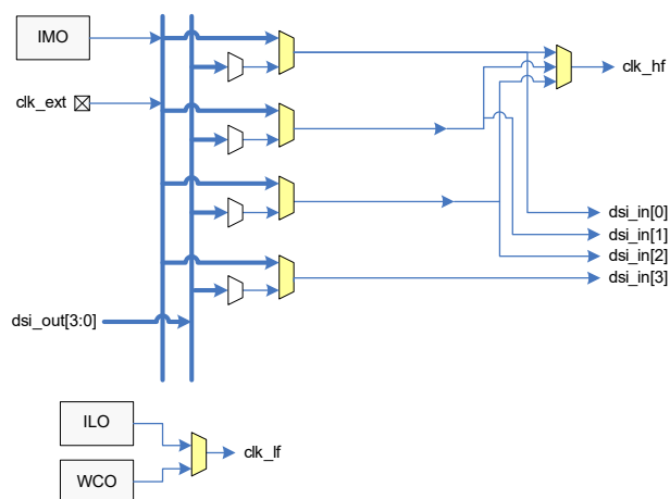
Figure 2. PSoC 4100M MCU Clocking Architecture
