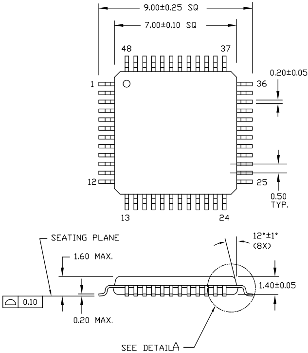
Figure 6. 48-Pin 7 × 7 × 1.4 mm TQFP Package Outline
