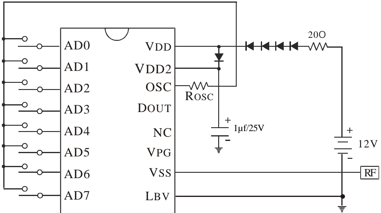
PT2283 (16 Pin)
