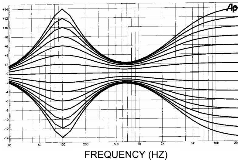
Typical Tone Response
