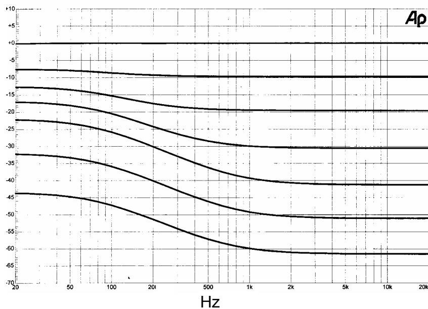
Loudness vs Volume Attenuation Frequency Response ( C_{10}=C_{11}=100\text{nF} )
