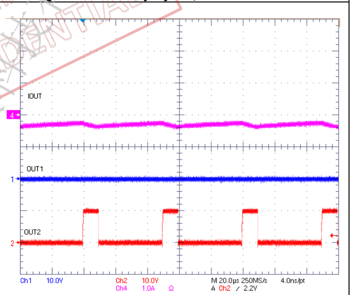
Figure 11. 20% Duty Cycle , Reverse Direction
