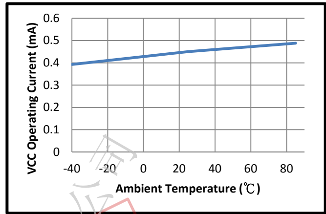
Figure 5. I_{VCC} vs T_A (50KHz PWM)
