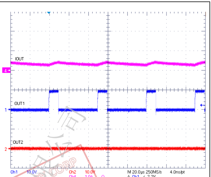
Figure 9. 20% Duty Cycle , Forward Direction
