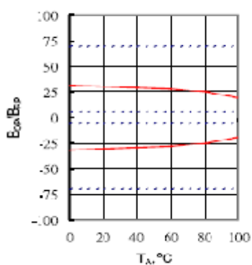
B_{OP}, B_{RP} versus temperature
