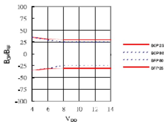
B_{OP}, B_{RP} versus supply voltage
