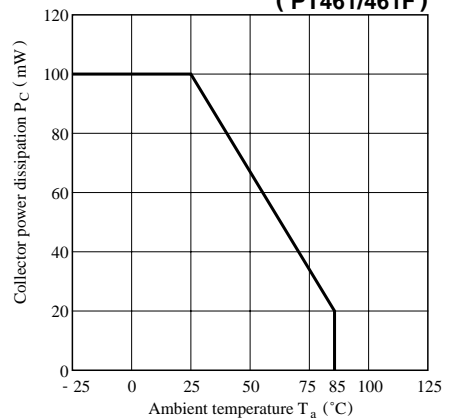
Fig. 1-b Collector Power Dissipation vs. Ambient Temperature (PT461/461F)
