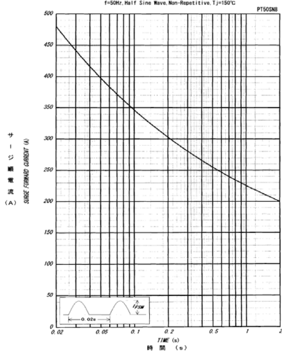
サージ順電流定格 SURGE CURRENT RATINGS f=50Hz, Half Sine Wave, Non-Repetitive, T j =150°C
