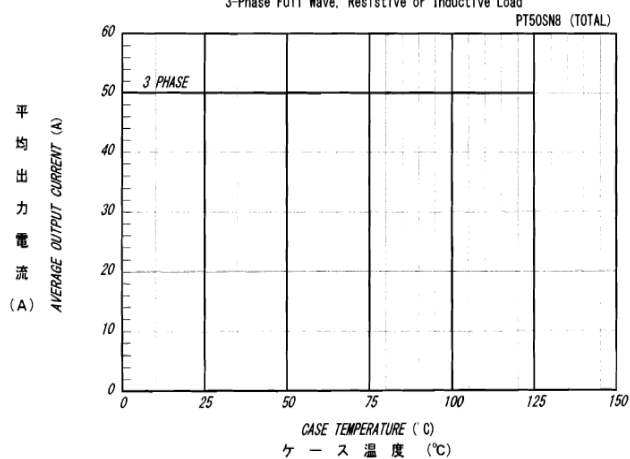
平均出力電流－ケース温度定格 AVERAGE OUTPUT CURRENT VS. CASE TEMPERATURE 3-Phase Full Wave, Resistive or Inductive Load
