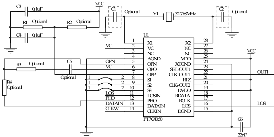
Normal Test Circuit
