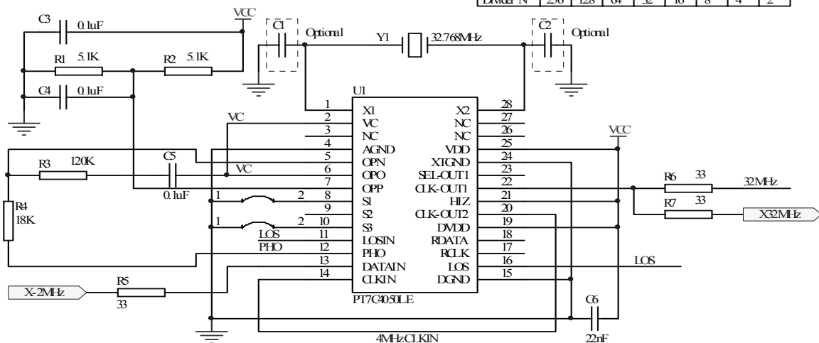
Application circuit for PT7C4050 Input: 2MHz Output: 32.768MHz
