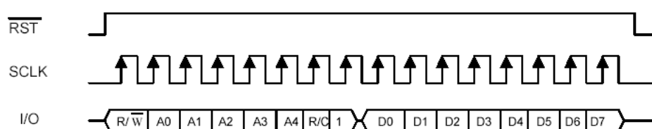
Figure 3 Single byte write
