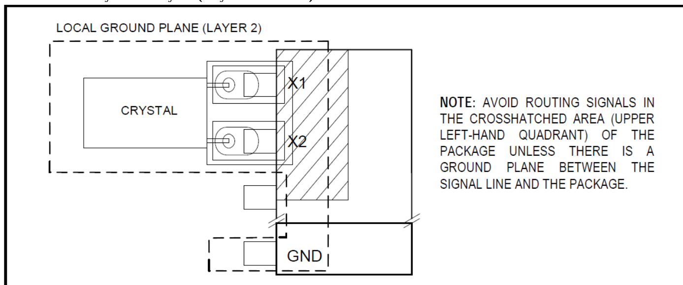
Figure 2 typical PC board layout for isolating the crystal and oscillator from noise
