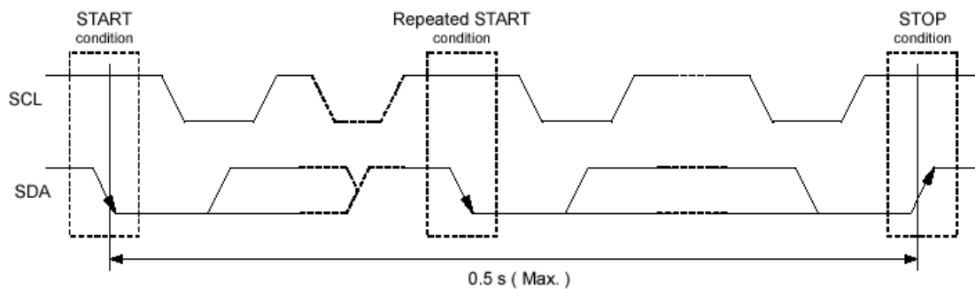
Fig3. Starting and stopping on I 2 C bus
