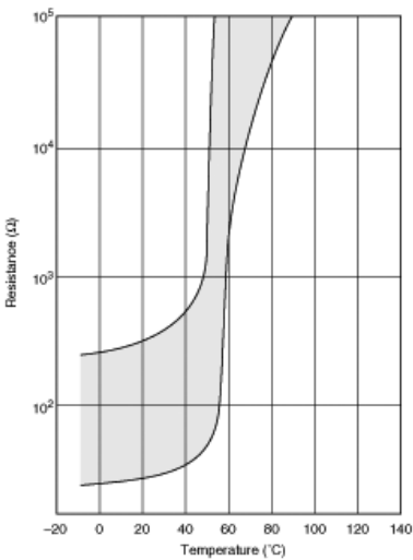
Resistance-Temperature Characteristics Range
