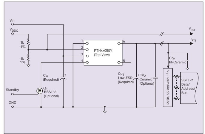
Figure 4 - Standard Application
