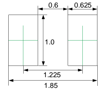
Recommended Soldering Pad
