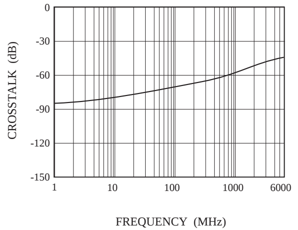
ANALOG CROSSTALK
