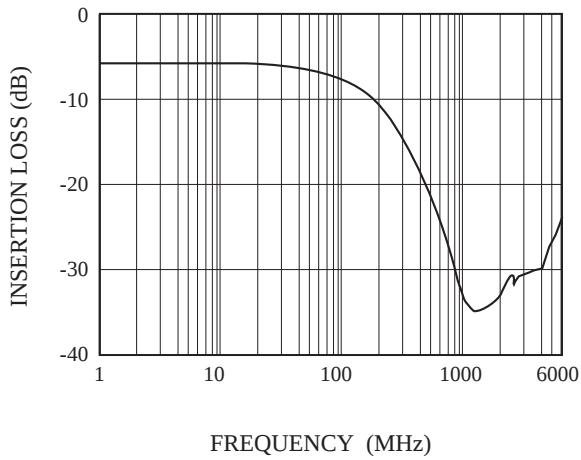
S_{21} - FREQUENCY
