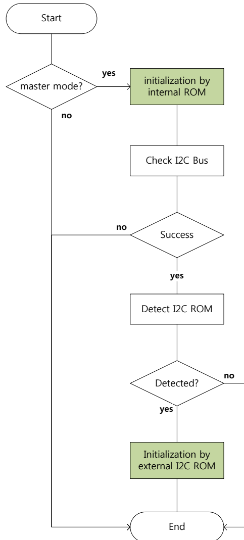
Figure 18 Initialization flow
