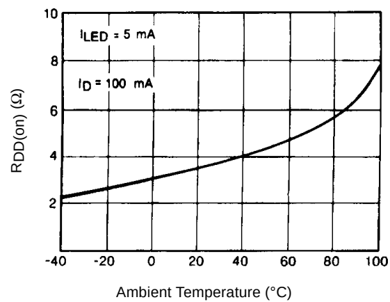
Figure 4. Typical On-Resistance
