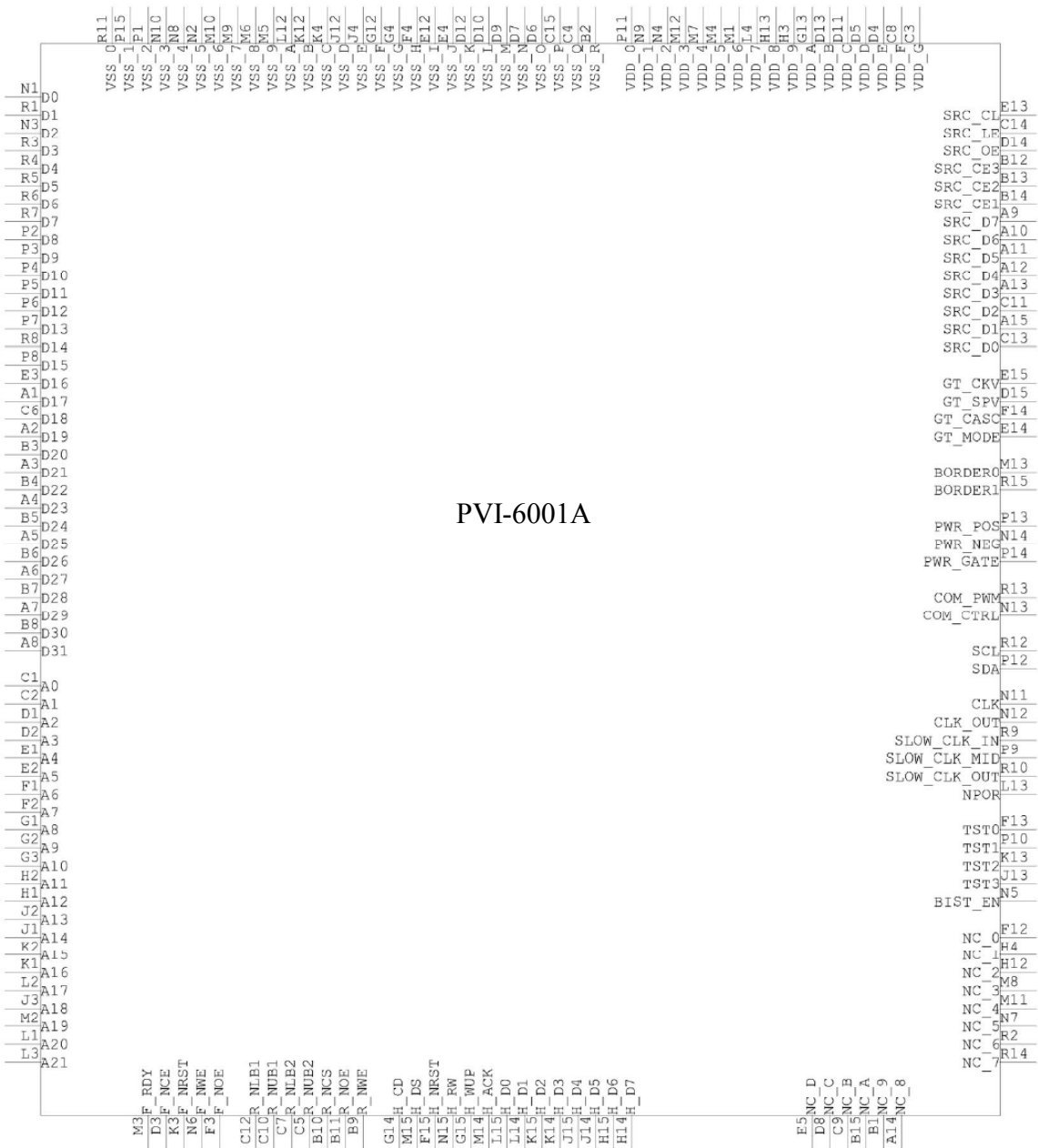
Figure 3.1 Symbol PVI-6001A
