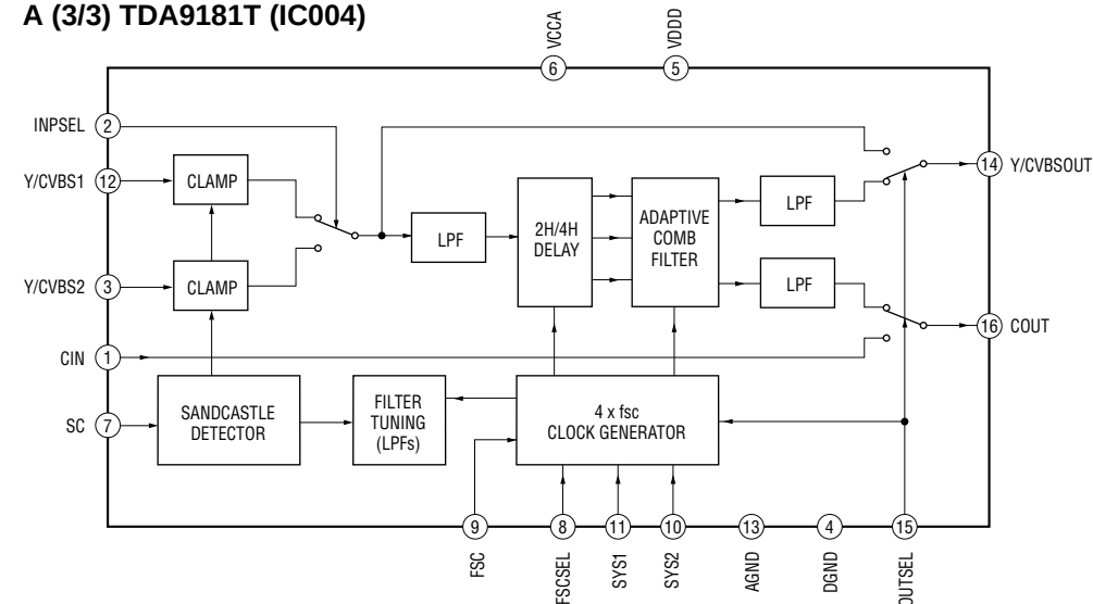
A (3/3) TDA9181T (IC004)
