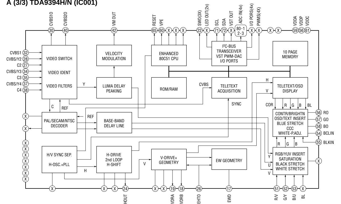
A (3/3) TDA9394H/N (IC001)
