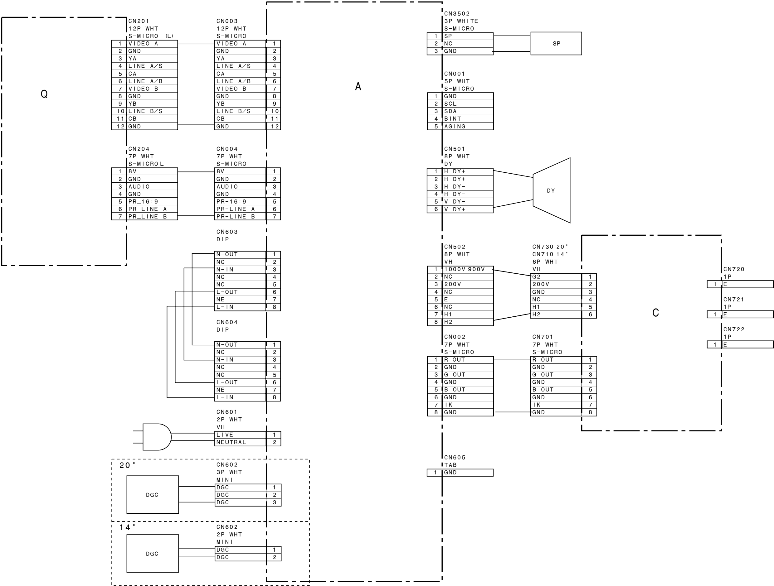
7-1. Frame Schematic Diagram
