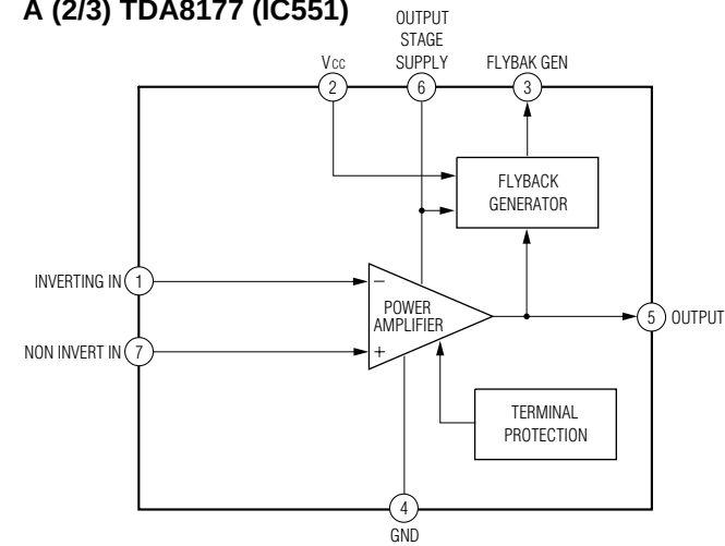
A (2/3) TDA8177 (IC551)
