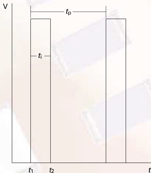
Rectangular Pulses
