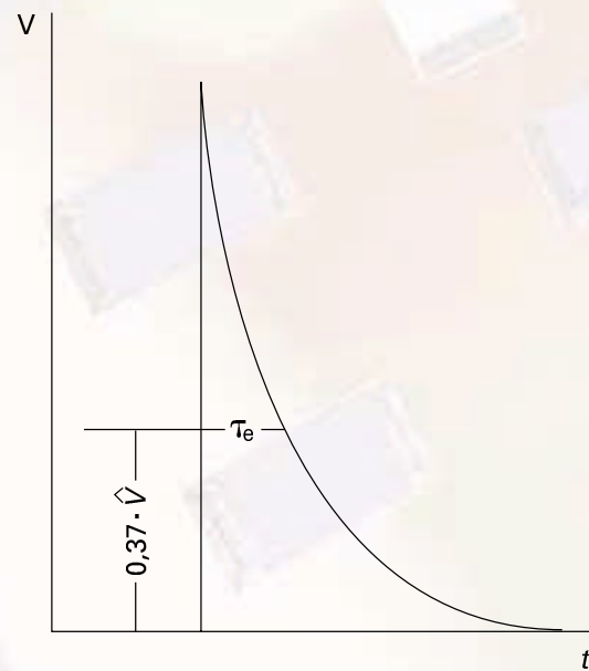
Exponential Pulse
