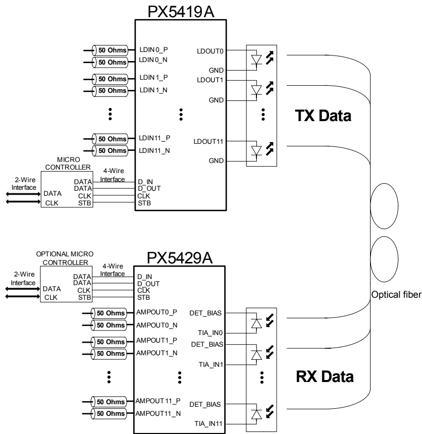
Figure 2: Application block diagram utilizing the PX5419A VCSEL driver and the PX5429A optical receiver
