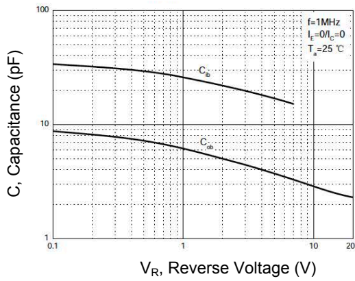
Figure 7. Capacitance Characteristics
