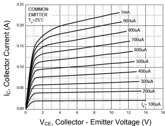
Figure 1. Static Characteristics
